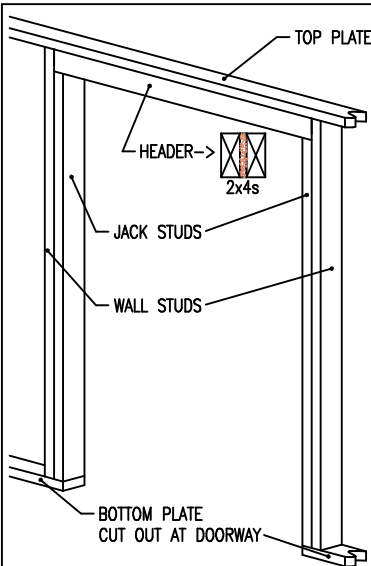
TYPICAL DOOR FRAMING
